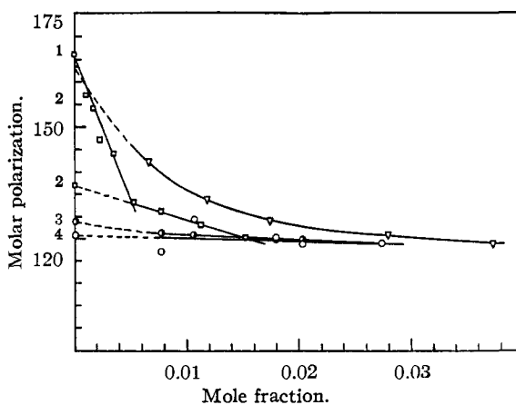
Fig. 2.—Ethyl benzoate:
